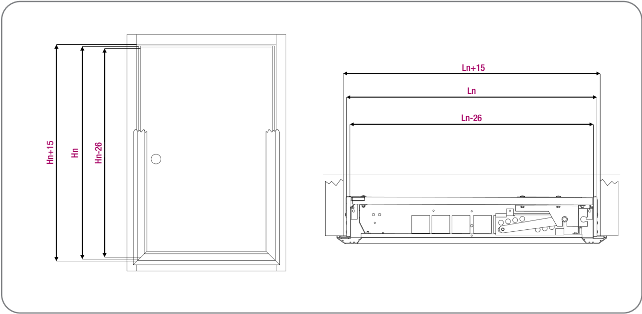
Free area table (SDK and SDK-PANEL without grid)
